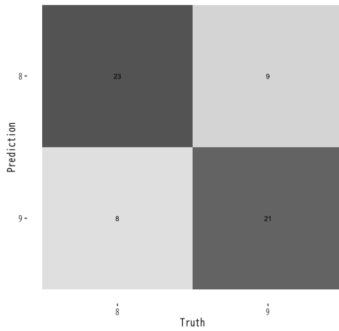
Figure 3: 線形判別の混同行列
