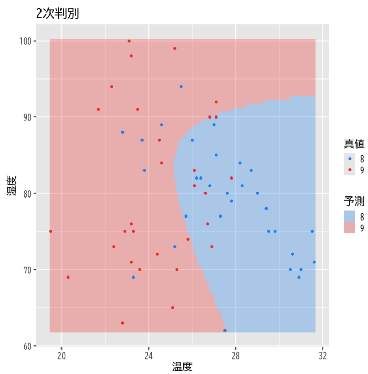
Figure 2: 2次判別
