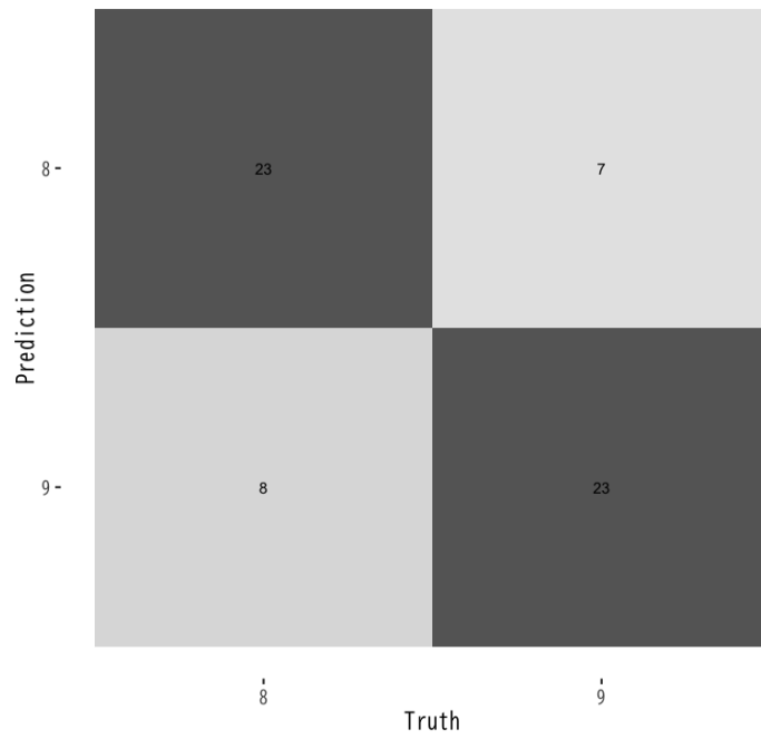
Figure 4: 2次判別の混同行列
