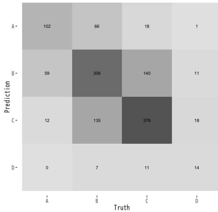
Figure 9: 訓練誤差
