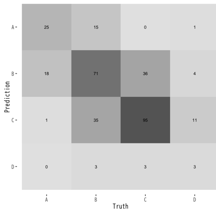
Figure 10: 予測誤差
