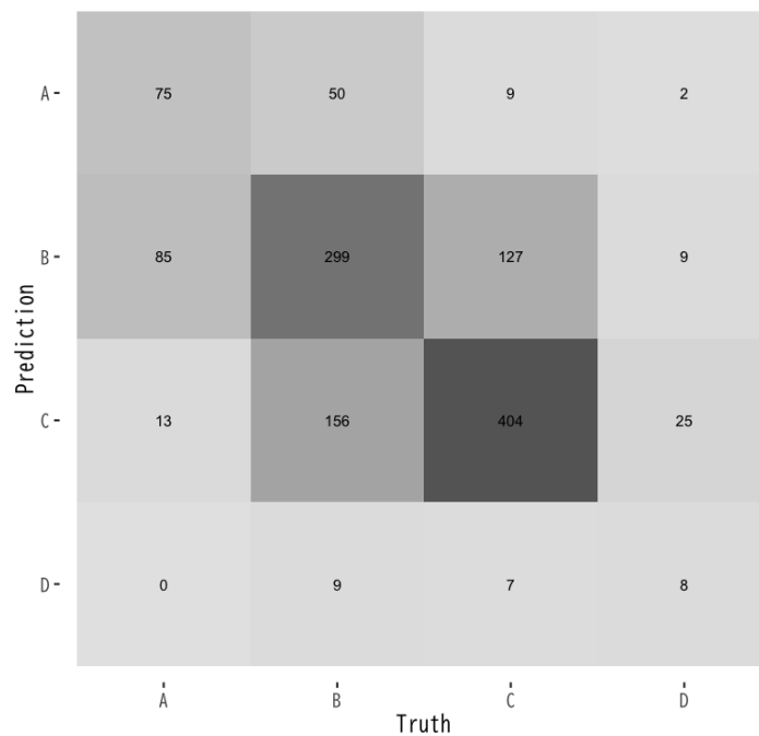
Figure 7: 訓練誤差
