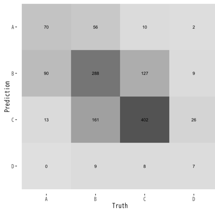
Figure 11: 線形判別
