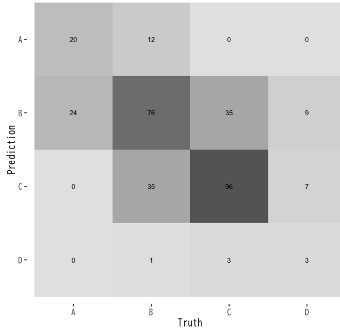
Figure 8: 予測誤差
